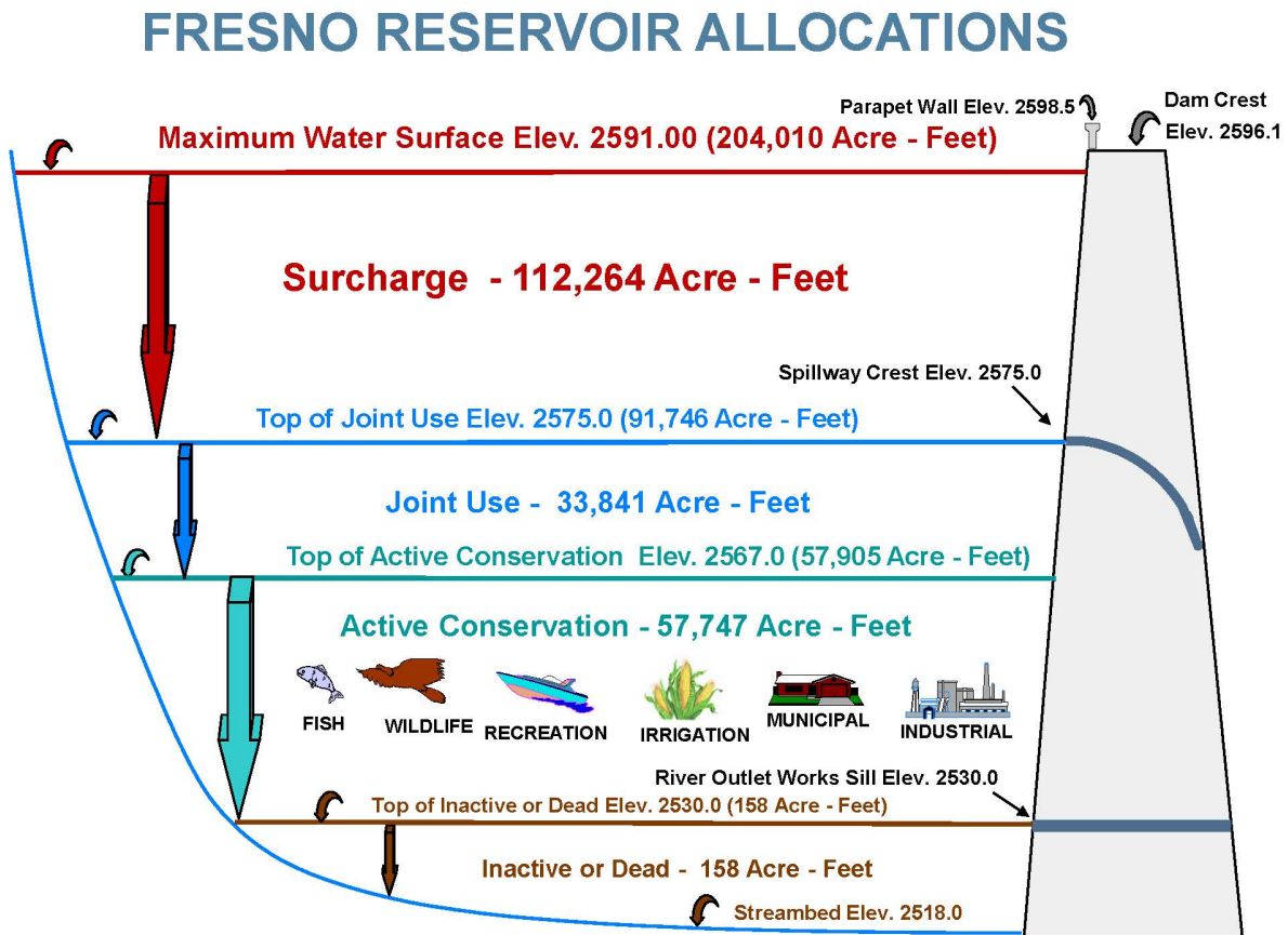
Figure 2: Fresno Reservoir Allocations
